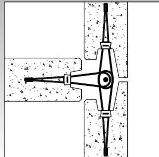
Fig 3: End Connection with crosswall.
