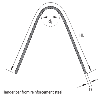
Hanger bar from reinforcement steel
